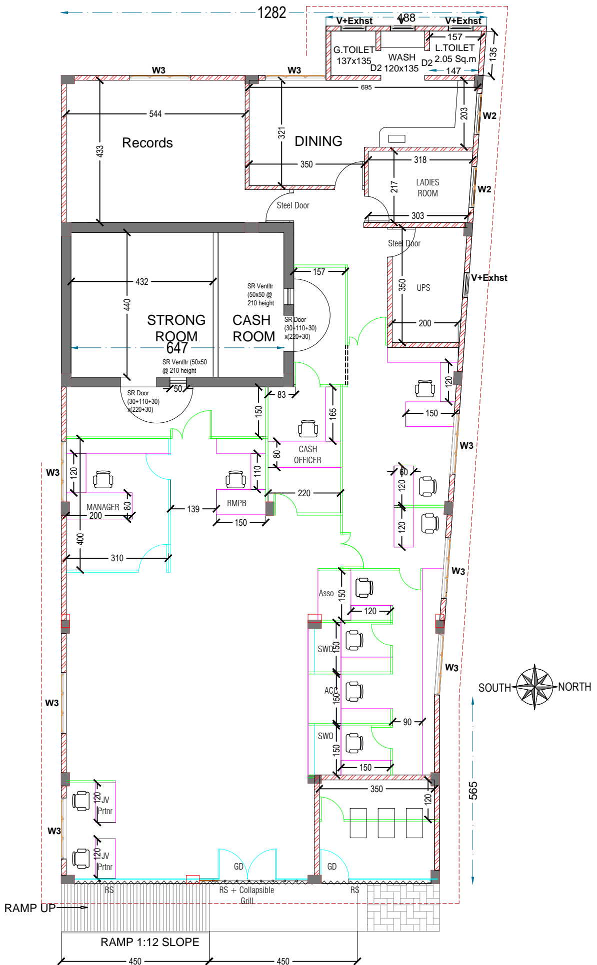
REVISED LAYOUT PLAN - KARIMKUNNAM BRANCH
